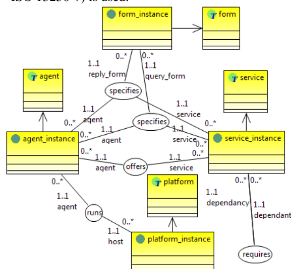
In Figure 4 the agents and their offered services are described. When the agent starts to run, a log entry is added containing the reference to the running platform. It then specifies a service which usually has a query form and a reply form. Note that the actual fields in the forms are described as occurrences of the form instances. The dependencies between the services may be defined as well at that point (i.e. in order to provide a map of high concentration zones, weather report, concentration measurements and information about the source leak
